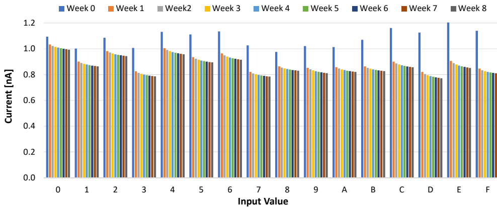
Figure 6: Simulated static current change for different aging duration and input stimuli.
